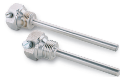
Example: Stainless steel sleeve for temperature sensor with installation length 85 mm and 120 mm with side clamping screw
